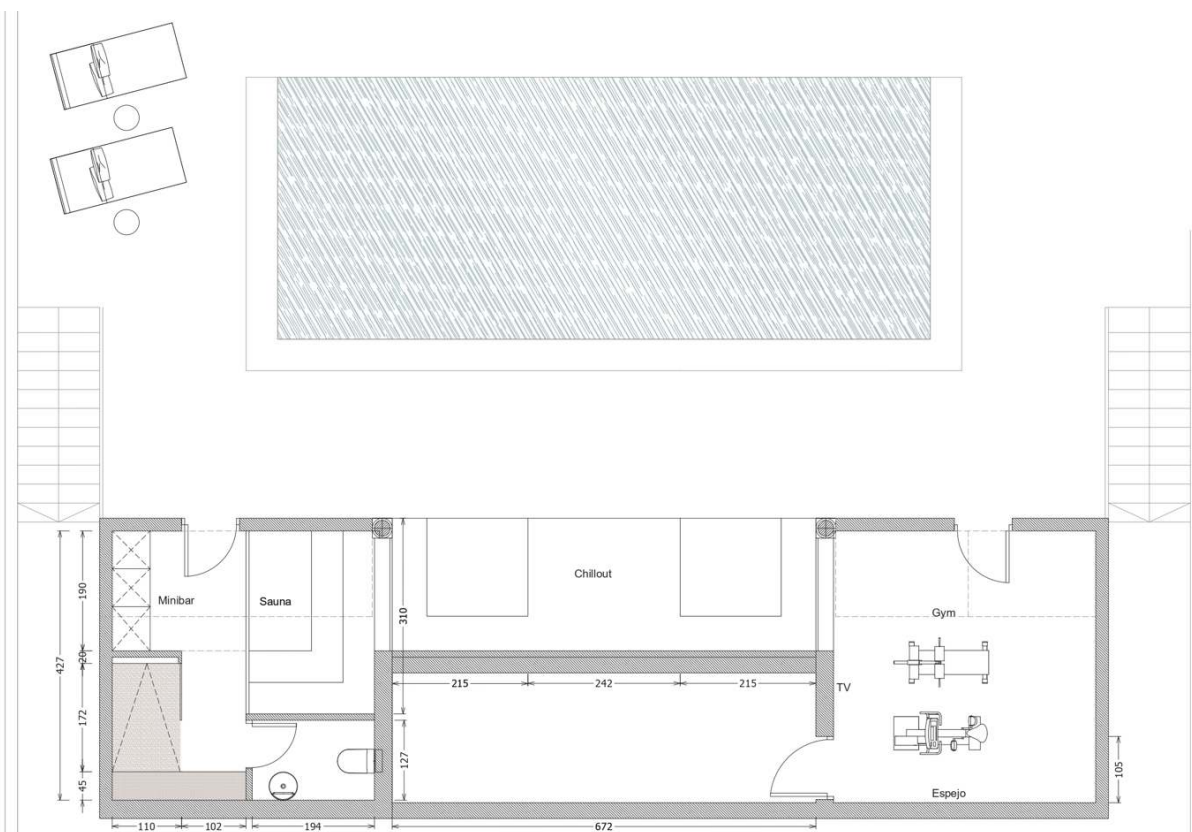
adm INTERIOR DESIGNER: Jazmin Lopez Becker | jlopez@adm-design.com PROJECT: PISO 5 | HORNOSSET - ANDRATX CLIENT: Watercress Friends FLOOR: PLANTA SEGUNDA CONTENT: PLANTA SEGUNDA SCALE: 1:50 DATE: 09/02/2022 A3
