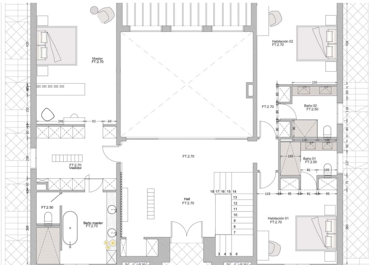
adm INTERIOR DESIGNER: Jazmin Lopez Becker | jlopez@adm-design.com PROJECT: PISO 5 | HORNOSSET - ANDRATX CLIENT: Watercress Friends FLOOR: PLANTA PRIMERA CONTENT: PLANTA PRIMERA SCALE: 1:50 DATE: 09/02/2022 A3
