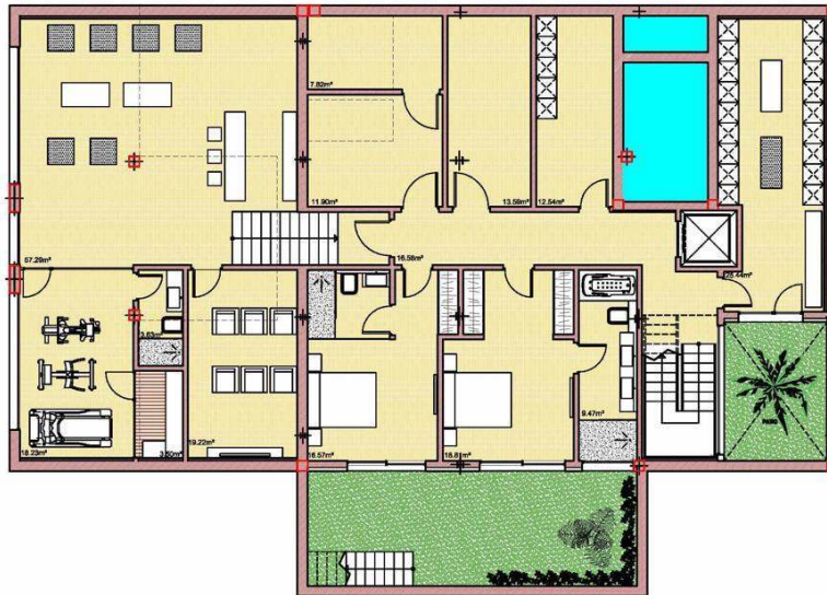
BASEMENT E: 1/100
